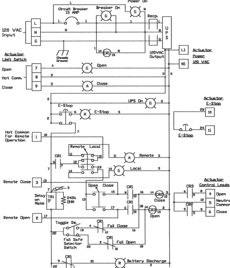
BUPS Electrical Schematic
